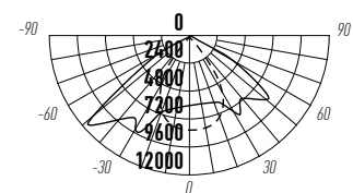
PSL 05-2 100W
