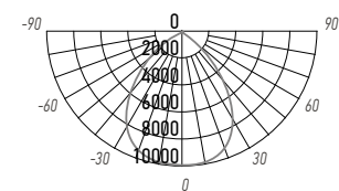
PFL-S4 150W
