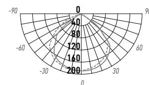
PFL SOLAR 02 50
