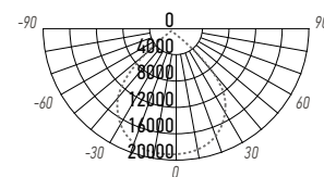
PFL-S5 200W
