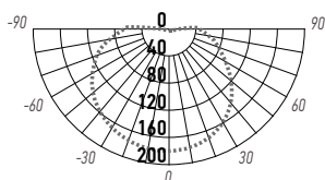
MTR16 3010 10W
