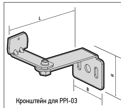
PPI-03 200W
