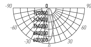
PFL-SPORT 02 750W
